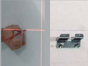
Anchors location
